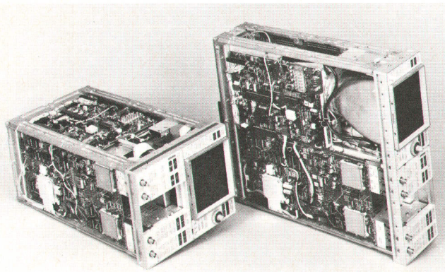
Fig. 1. Models 1980A (left) and 1980B are designed to have as many components and boards in common as possible.
