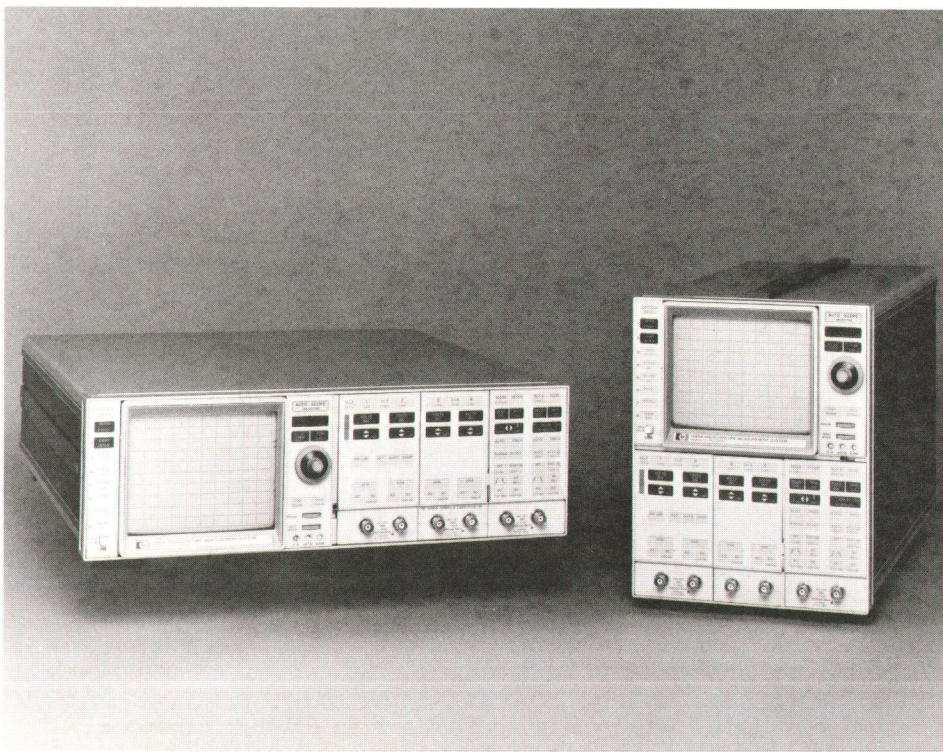
Fig. 1. Designed for use in automated systems, Model 1980A/B Oscilloscope Measurement System is compatible with the HP-IB (IEEE 488). Among its features are Autoscope, which gives the user a display rapidly and automatically, and front-panel calibration. Options include digital waveform storage and measurement sequence memory. (r) Model 1980A. (l) Model 1980B.
