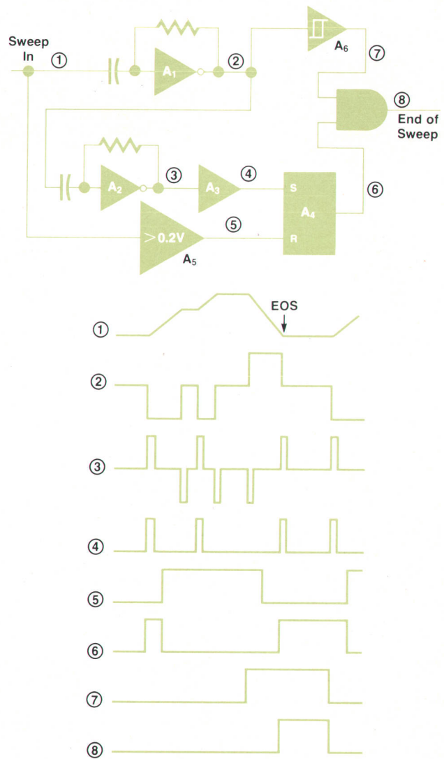
Fig. 7. End-of-sweep detection in lock-and-roll mode.
