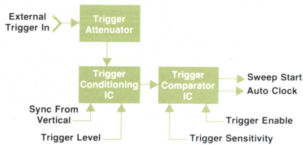
Fig. 9. 1980A/B trigger system block diagram.
